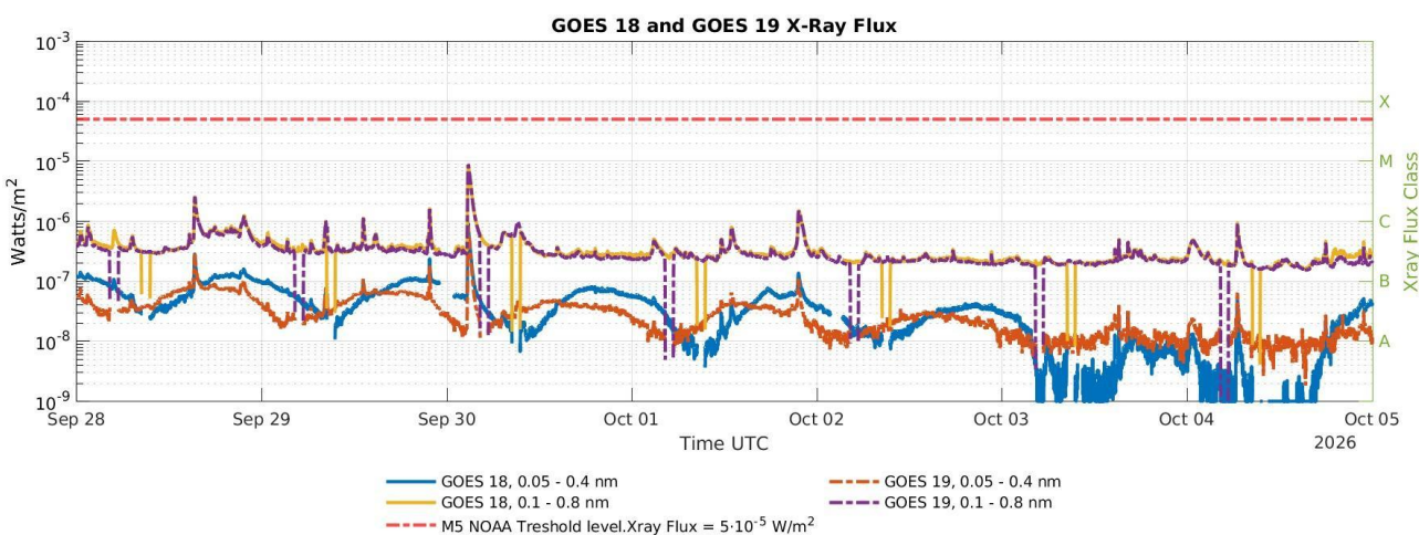
Figure 3: X-ray flux coming from the Sun as measured by NOAA GOES satellite constellation.
