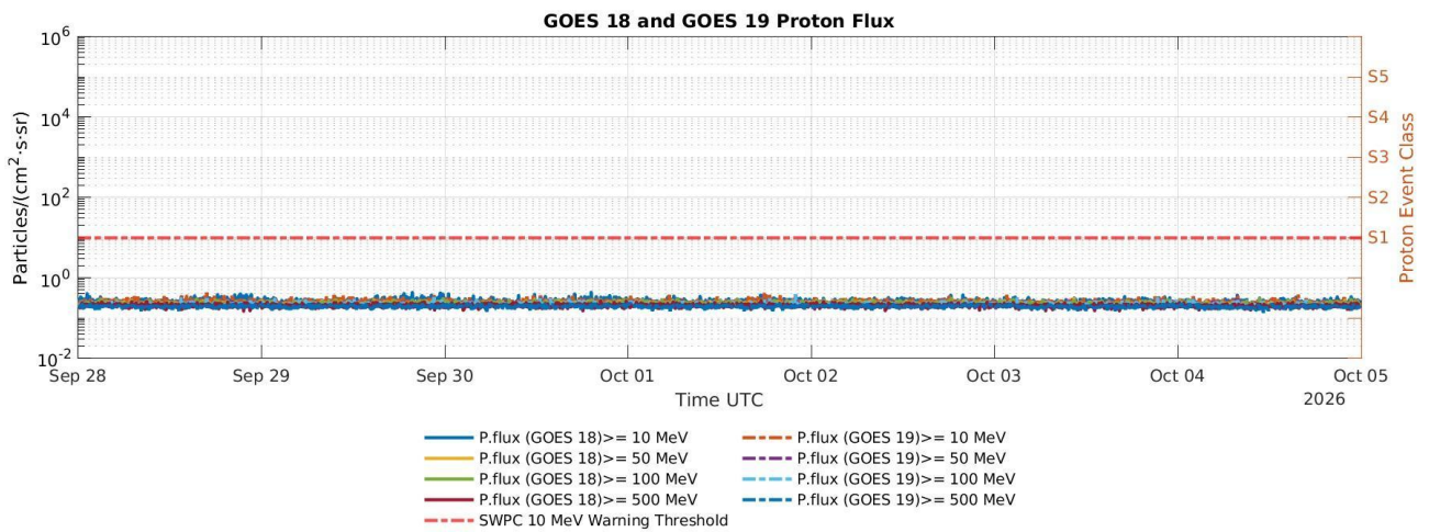
Figure 4: Solar proton's flux measured by NOAA GOES satellite constellation.
