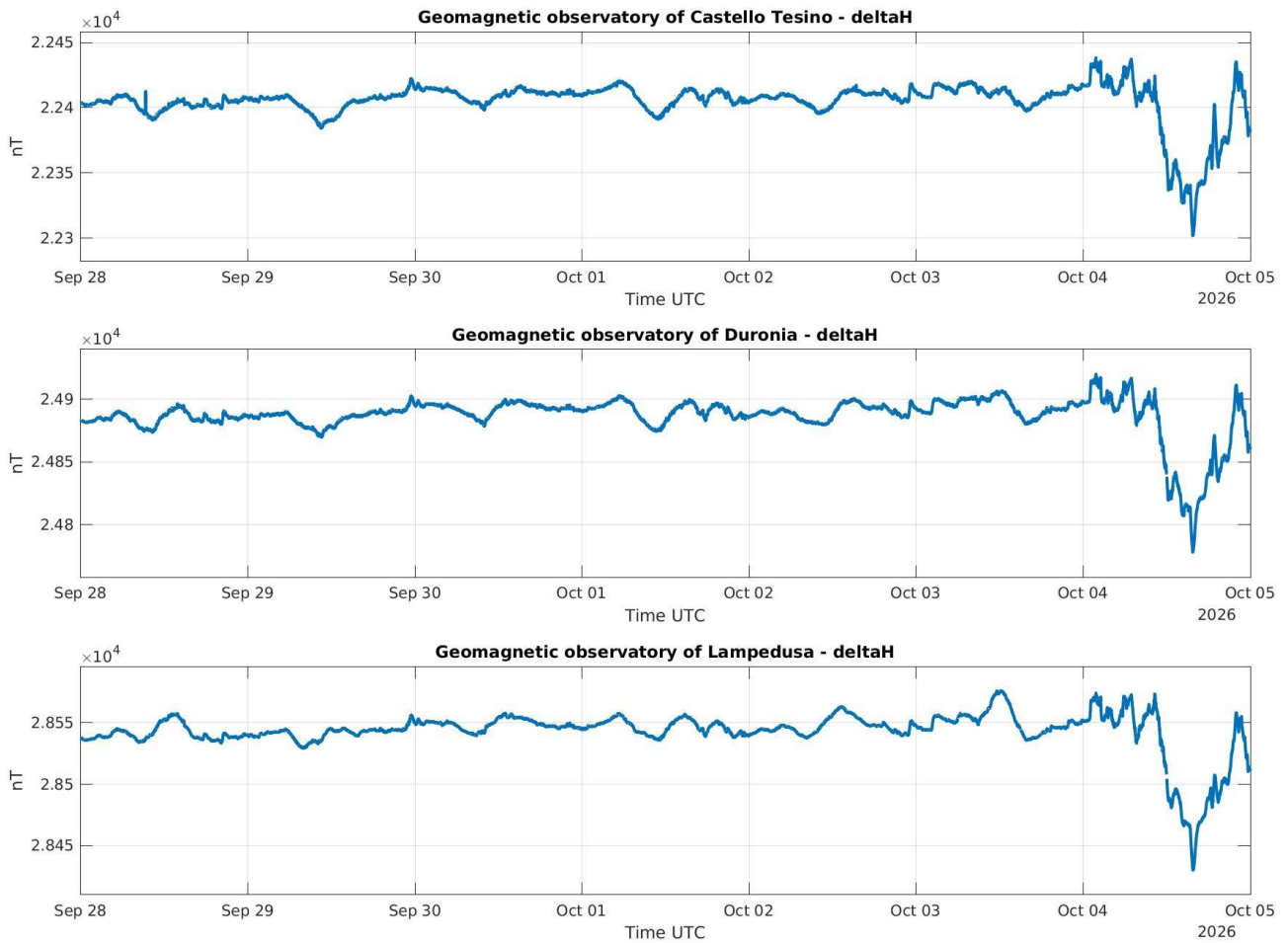
Figure 13: Magnetograms showing the variation of the horizontal component of the Earth's magnetic field at the Italian geomagnetic observatories (Castello Tesino, Durnia and Lampedusa from top to bottom).
