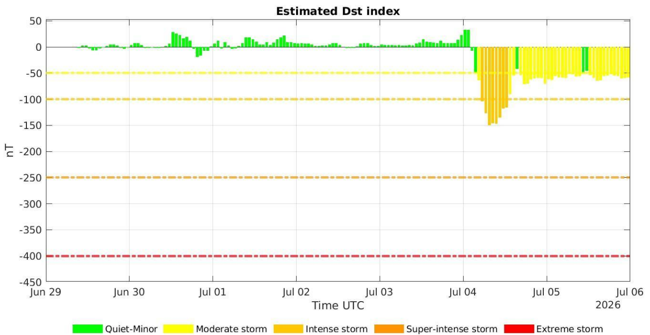
Figure 16: Histogram of Dst index taken from NOAA. Coloured bars indicate the intensity of the disturbance of the ring current, according to the corresponding thresholds.
