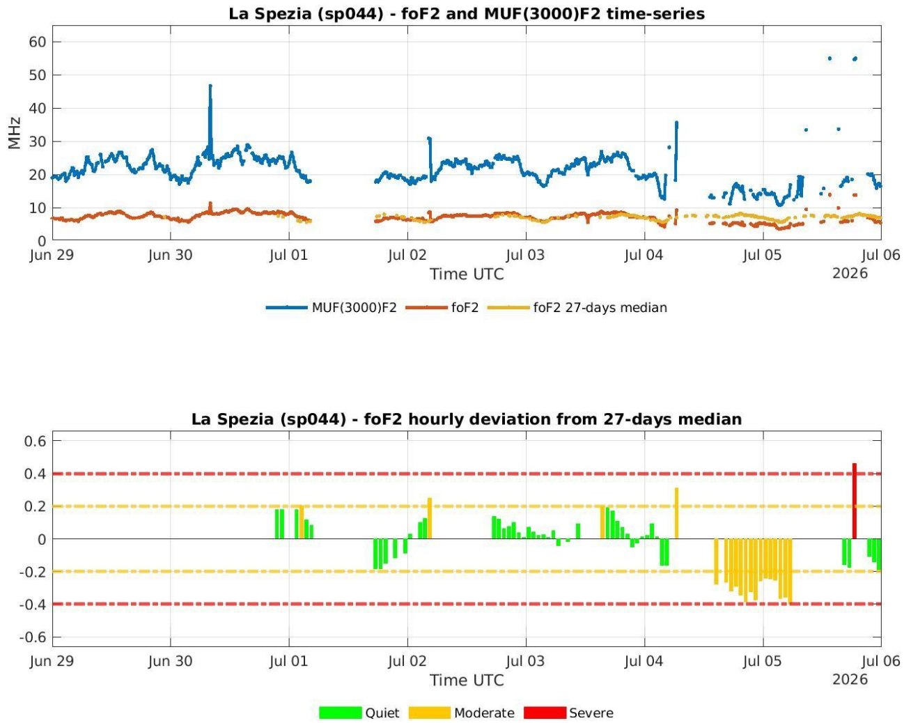
Figure 6: HF data from the INGV ionospheric observatory of La Spezia. Top panel: foF2 (orange), corresponding median over the previous 27 days (yellow), and MUF(3000)F2 (blue); Bottom panel: foF2 hourly-averaged relative deviation from 27-days median, with colors (green, yellow and red) associated to the severity of the perturbation, according to the \pm 0.2 and \pm 0.4 thresholds reported with horizontal yellow and red dashed lines, respectively.
