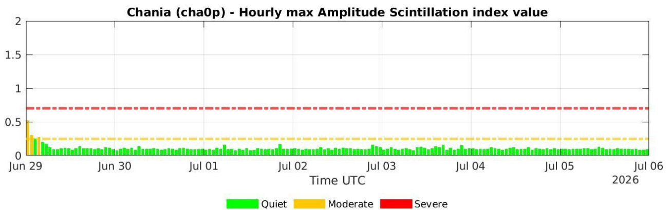
Figure 12: Same as Figure 10 for the data from the INGV receiver for GNSS scintillation located in Chania.
