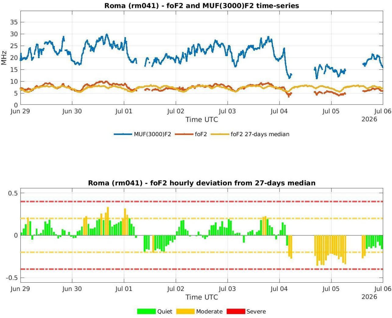
Figure 7: Same as Fig. 6 for the HF data from the INGV ionospheric observatory of Roma.
