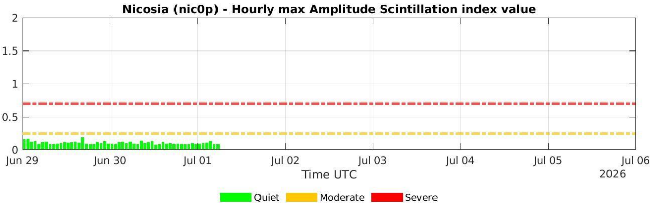
Figure 11: Same as Figure 10 for the data from the INGV receiver for GNSS scintillation located in Nicosia.
