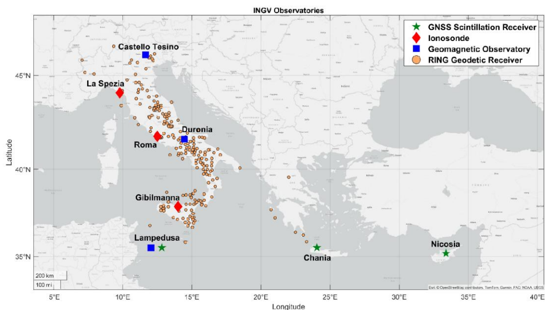
Figure 1: Locations of the INGV observatories and measuring stations which acquire data useful for Space Weather purposes.
