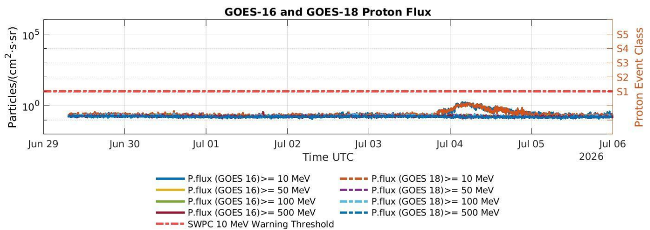
Figure 4: Solar proton's flux measured by GOES-16 and GOES-18 NOAA satellites.
