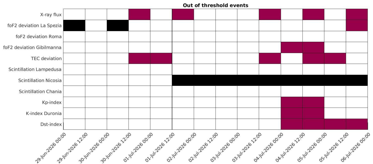
Figure 2: Summary of measurements which reported out-of-threshold events (red boxes) and lack of data (black ones) during the week.
