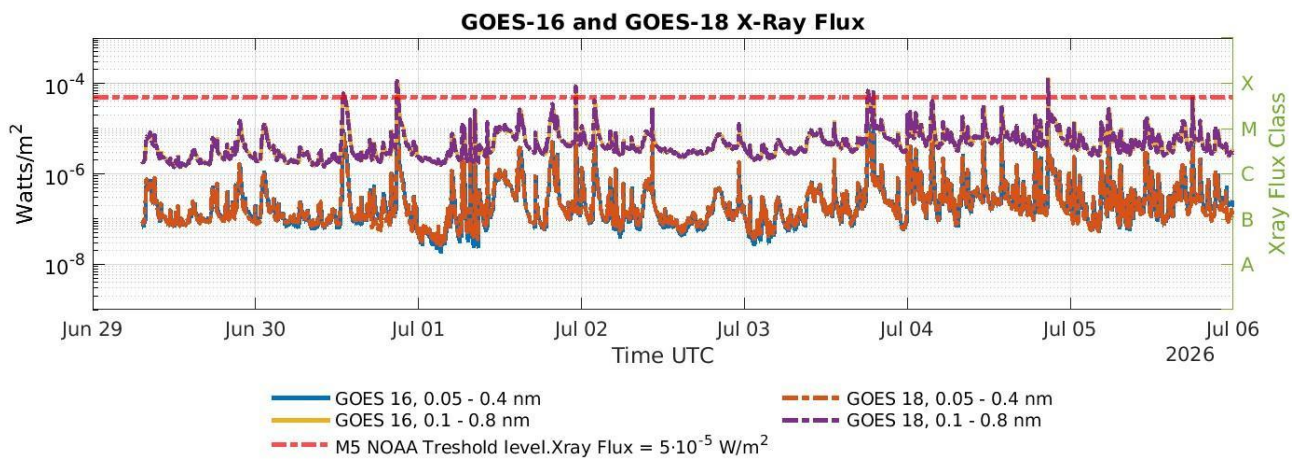
Figure 3: X-ray flux coming from the Sun as measured by GOES-16 and GOES-18 NOAA satellites.
