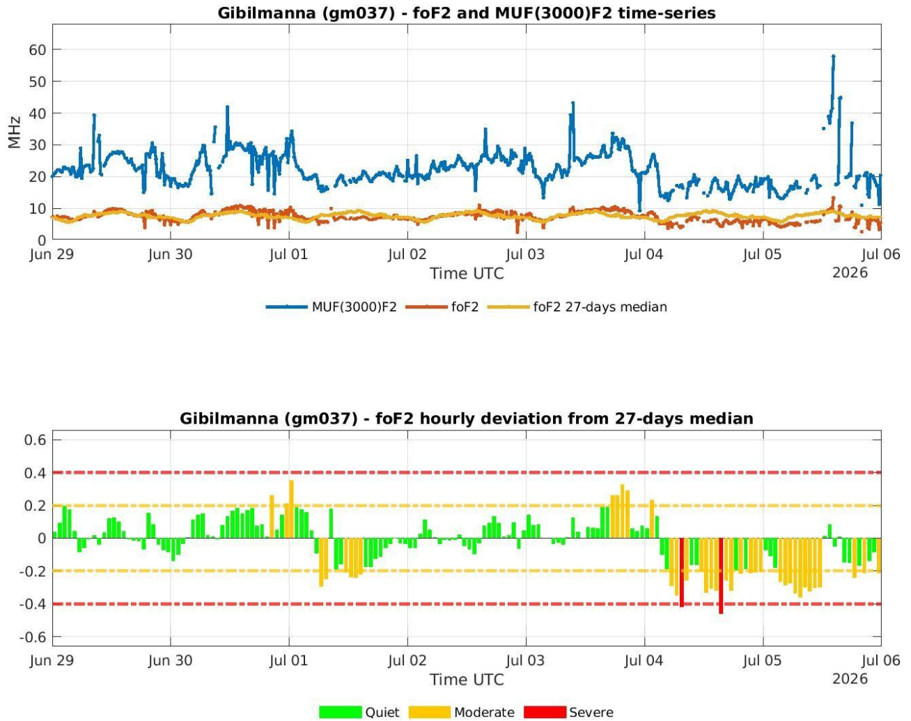
Figure 8: Same as Fig. 6 for the HF data from the INGV ionospheric observatory of Gibilmanna.
