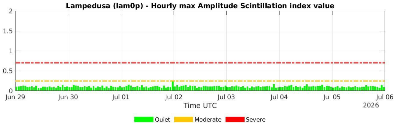
Figure 10: S4 hourly maximum values recorded by the INGV receiver for GNSS scintillation located in Lampedusa, with colors (green, yellow and red) associated to the severity of the scintillation, according to the 0.25 and 0.7 thresholds reported with horizontal yellow and red dashed lines, respectively.
