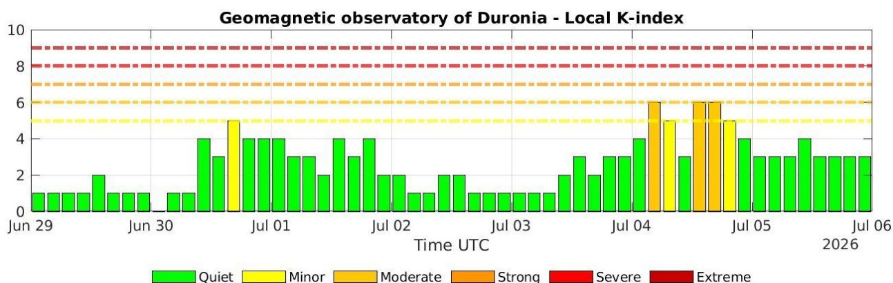
Figure 15: As in Figure 14, histogram of local K index based on the magnetic field recorded at Duronia geomagnetic observatory.
