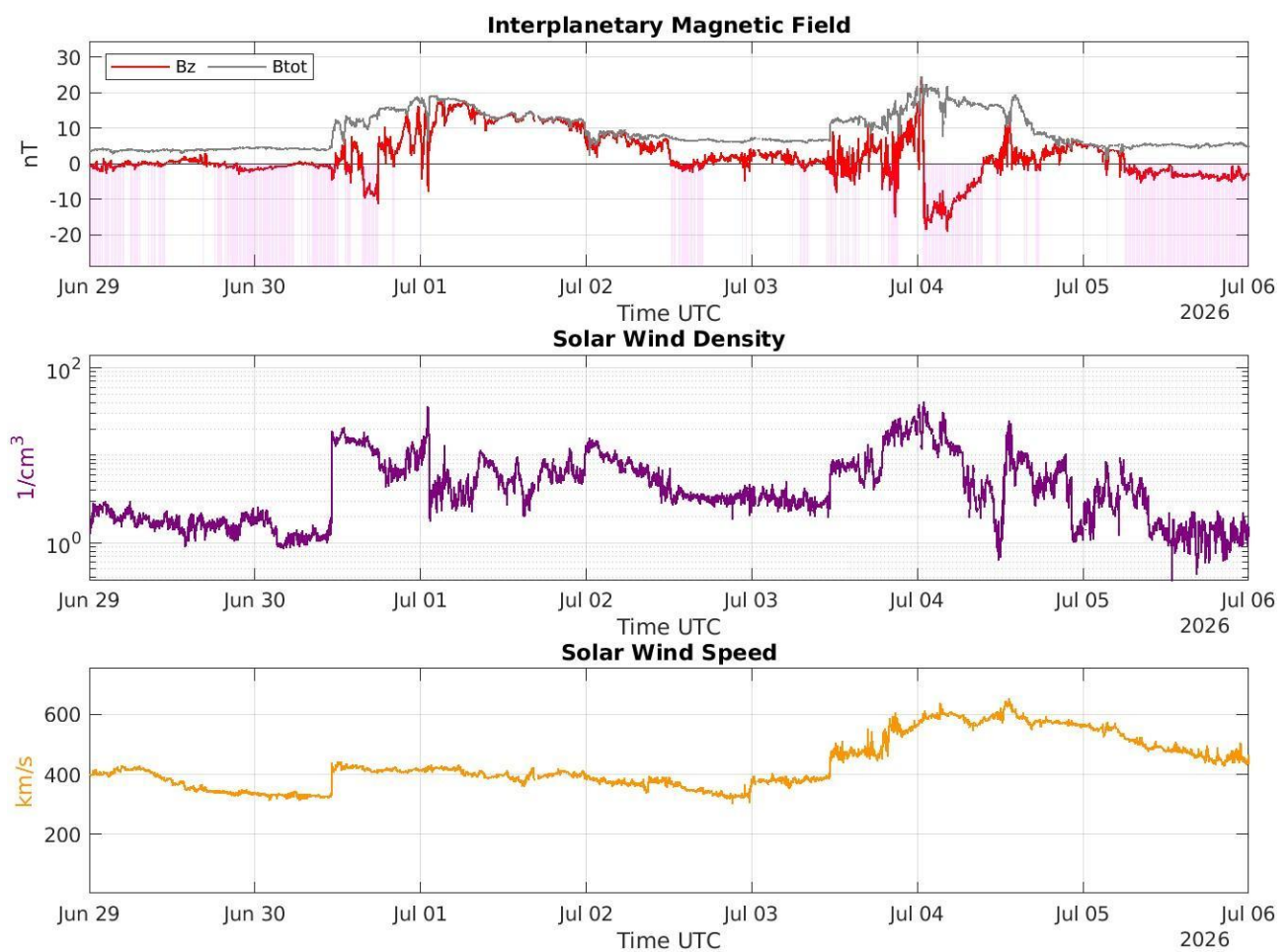
Figure 5: Top panel: Interplanetary Magnetic Field B_z (red) component and total field (black); Middle panel: Solar Wind density; Bottom panel: Solar Wind speed. Measures come from NASA DISCVR spacecraft, or NASA ACE spacecraft if DISCVR data are not available.
