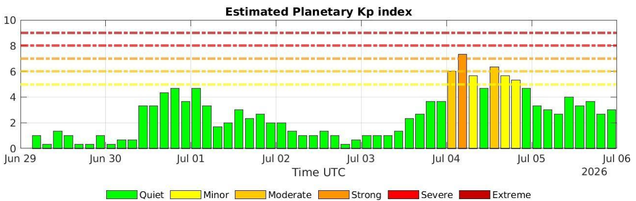
Figure 14: Histogram of Kp index released by NOAA. Coloured bars indicate the intensity of the global magnetic activity on Earth, according to the corresponding thresholds.
