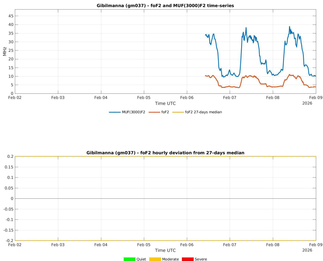
Figure 8: Same as Fig. 6 for the HF data from the INGV ionospheric observatory of Gibilmanna.
