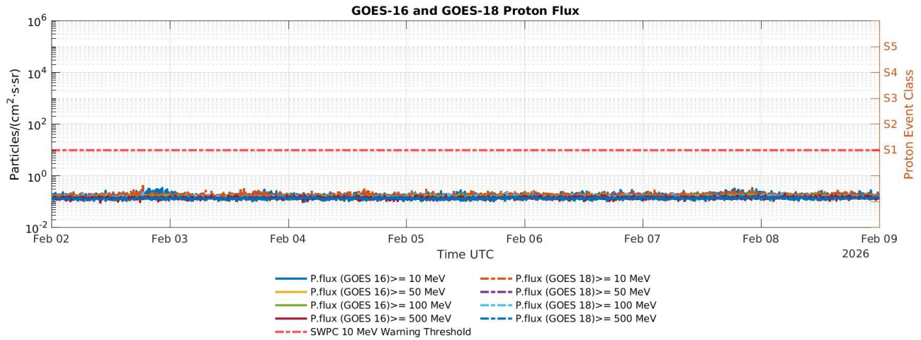
Figure 4: Solar proton's flux measured by GOES-16 and GOES-18 NOAA satellites.
