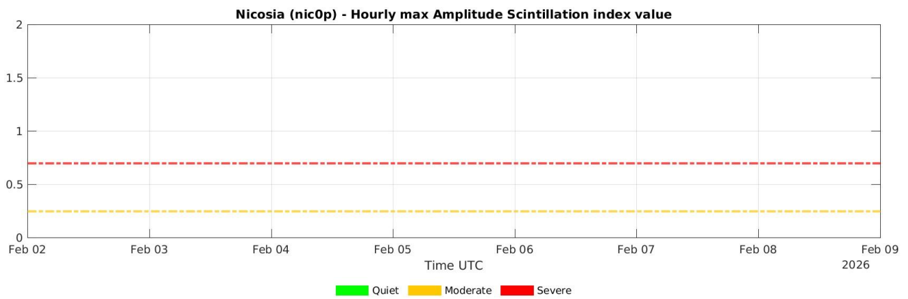
Figure 11: Same as Figure 10 for the data from the INGV receiver for GNSS scintillation located in Nicosia.
