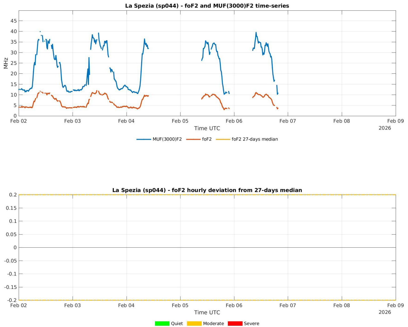
Figure 6: HF data from the INGV ionospheric observatory of La Spezia. Top panel: foF2 (orange), corresponding median over the previous 27 days (yellow), and MUF(3000)F2 (blue); Bottom panel: foF2 hourly-averaged relative deviation from 27-days median, with colors (green, yellow and red) associated to the severity of the perturbation, according to the \pm 0.2 and \pm 0.4 thresholds reported with horizontal yellow and red dashed lines, respectively.
