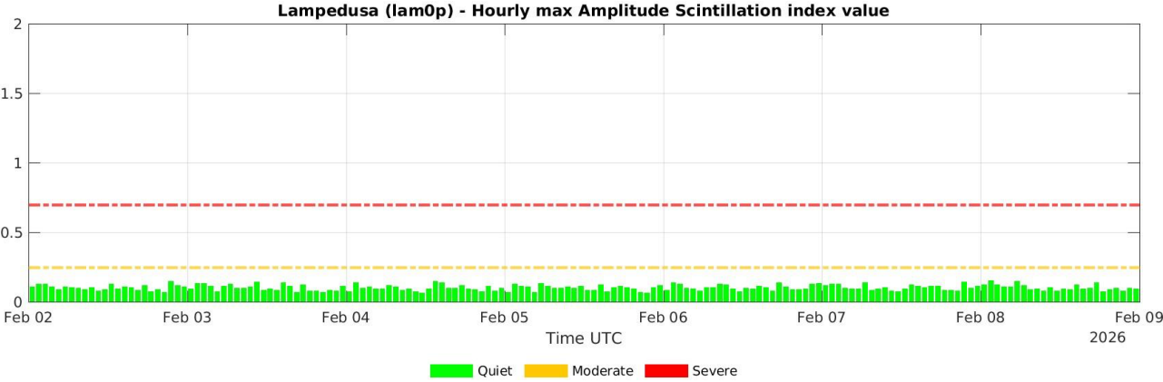
Figure 10: S4 hourly maximum values recorded by the INGV receiver for GNSS scintillation located in Lampedusa, with colors (green, yellow and red) associated to the severity of the scintillation, according to the 0.25 and 0.7 thresholds reported with horizontal yellow and red dashed lines, respectively.
