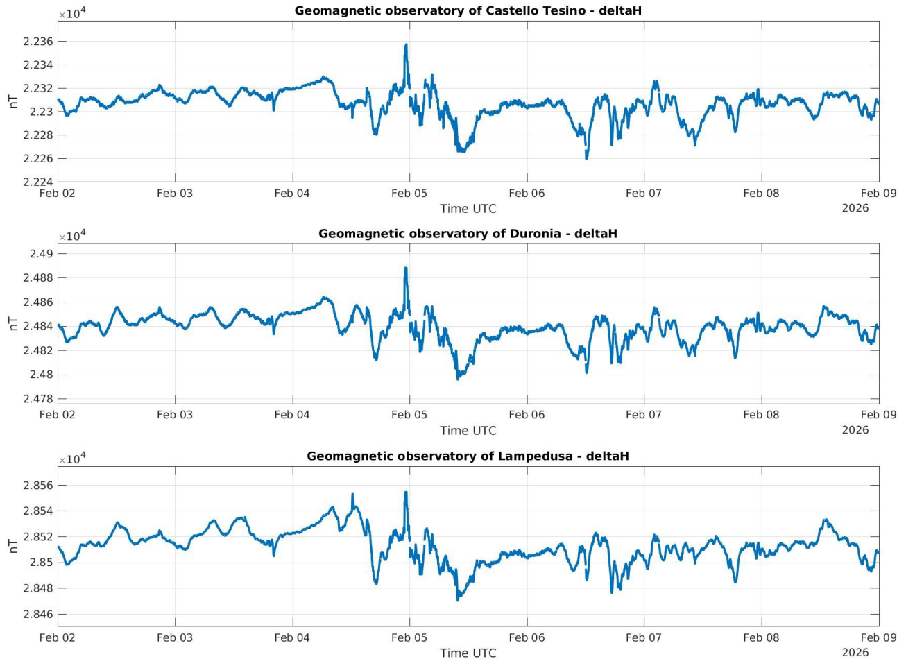
Figure 13: Magnetograms showing the variation of the horizontal component of the Earth's magnetic field at the Italian geomagnetic observatories (Castello Tesino, Duronia and Lampedusa from top to bottom).
