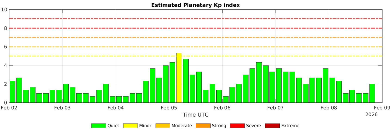
Figure 14: Histogram of Kp index released by NOAA. Coloured bars indicate the intensity of the global magnetic activity on Earth, according to the corresponding thresholds.
