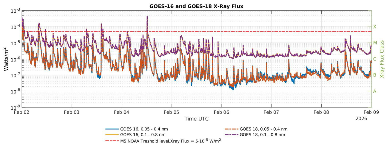
Figure 3: X-ray flux coming from the Sun as measured by GOES-16 and GOES-18 NOAA satellites.
