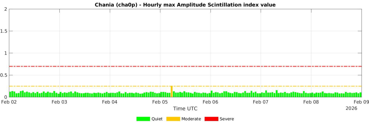
Figure 12: Same as Figure 10 for the data from the INGV receiver for GNSS scintillation located in Chania.
