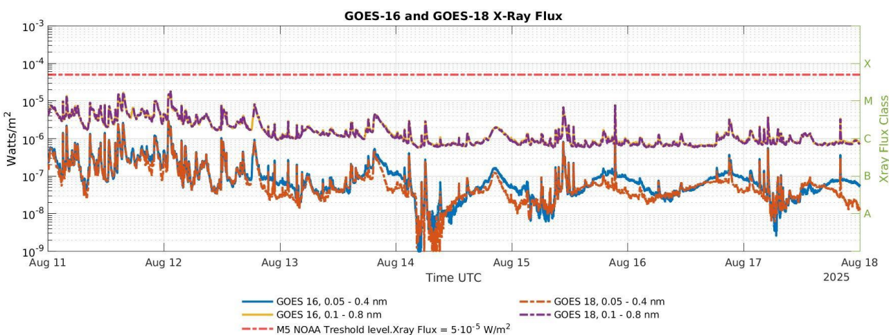
Figure 3: X-ray flux coming from the Sun as measured by GOES-16 and GOES-18 NOAA satellites.
