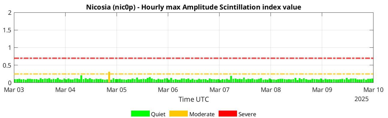
Figure 10: Same as Figure 9 for the data from the INGV receiver for GNSS scintillation located in Nicosia.
