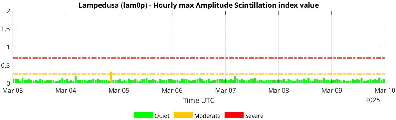
Figure 9: S4 hourly maximum values recorded by the INGV receiver for GNSS scintillation located in Lampedusa, with colors (green, yellow and red) associated to the severity of the scintillation, according to the 0.25 and 0.7 thresholds reported with horizontal yellow and red dashed lines, respectively.
