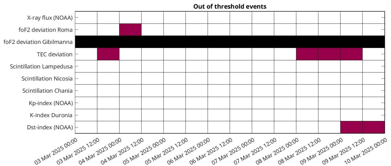
Figure 2: Summary of measurements which reported out-of-threshold events (red boxes) and lack of data (black ones) during the week.
