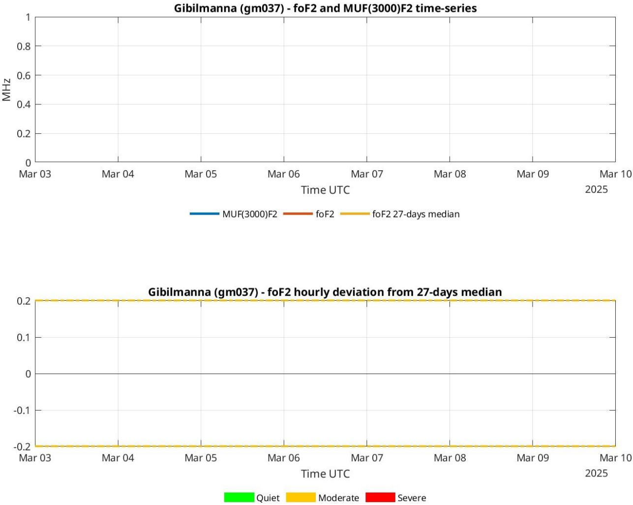
Figure 7: Same as Fig. 6 for the HF data from the INGV ionospheric observatory of Gibilmanna.
