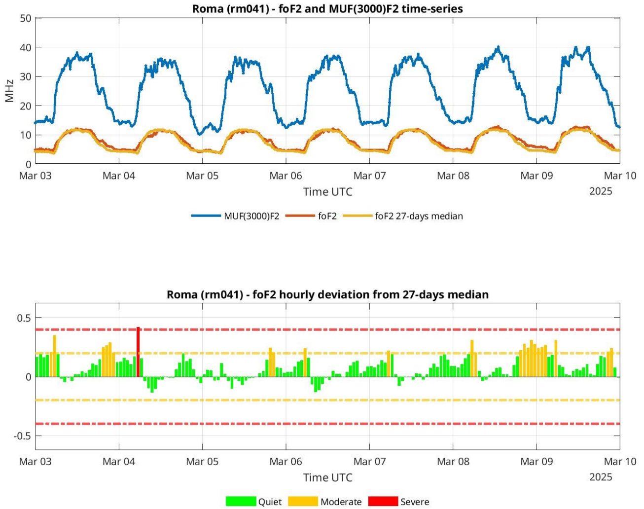
Figure 6: HF data from the INGV ionospheric observatory of Rome. Top panel: foF2 (orange), corresponding median over the previous 27 days (yellow), and MUF(3000)F2 (blue); Bottom panel: foF2 hourly-averaged relative deviation from 27-days median, with colors (green, yellow and red) associated to the severity of the perturbation, according to the \pm 0.2 and \pm 0.4 thresholds reported with horizontal yellow and red dashed lines, respectively.
