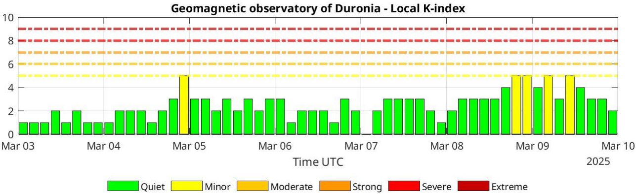
Figure 14: As in Figure 13, histogram of local K index based on the magnetic field recorded at Duronio geomagnetic observatory.
