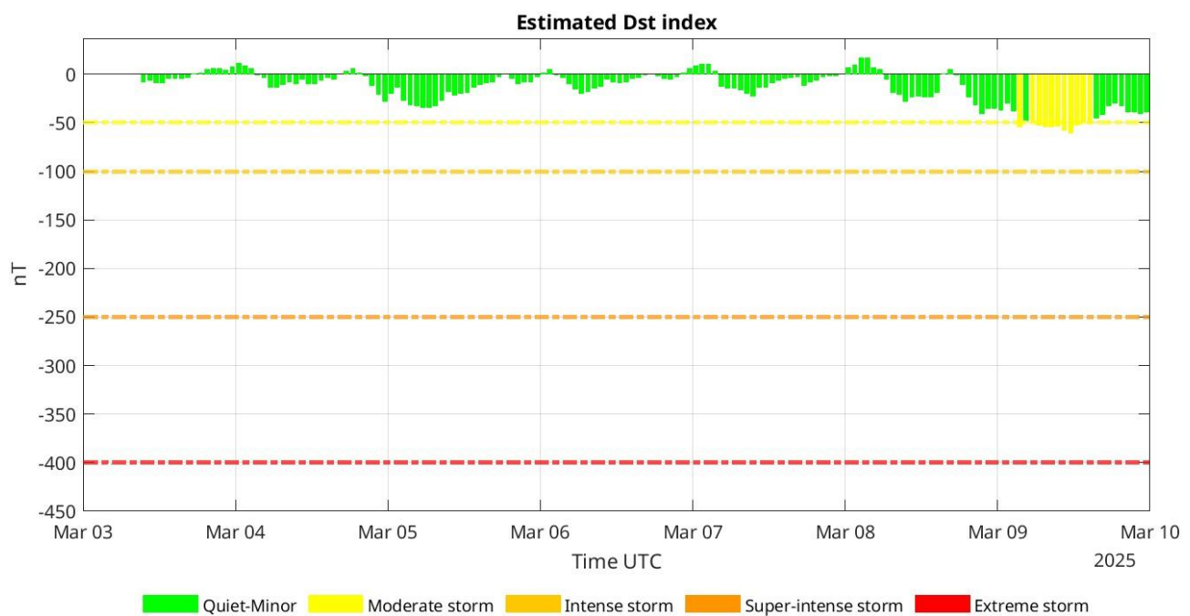
Figure 15: Histogram of Dst index taken from NOAA. Coloured bars indicate the intensity of the disturbance of the ring current, according to the corresponding thresholds.
