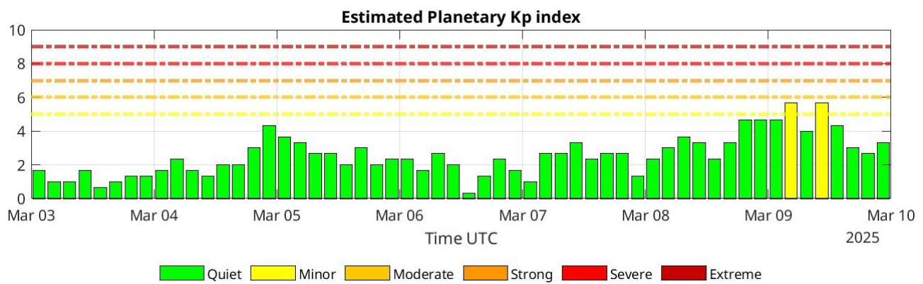
Figure 13: Histogram of Kp index released by NOAA. Coloured bars indicate the intensity of the global magnetic activity on Earth, according to the corresponding thresholds.
