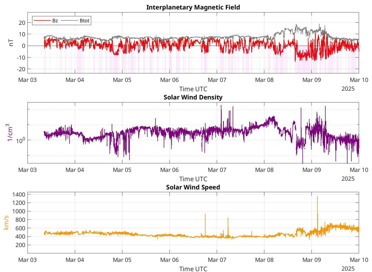
Figure 5: Top panel: Interplanetary Magnetic Field B_z (red) component e total field (black); Middle panel: Solar Wind density; Bottom panel: Solar Wind speed. Measures come from NASA DISCVR spacecraft, or NASA ACE spacecraft if DISCVR data are not available.
