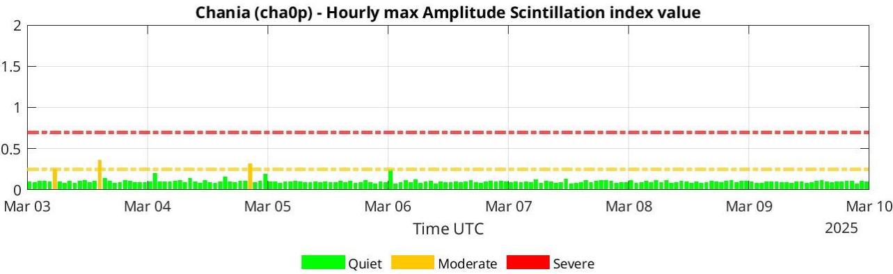
Figure 11: Same as Figure 9 for the data from the INGV receiver for GNSS scintillation located in Chania.
