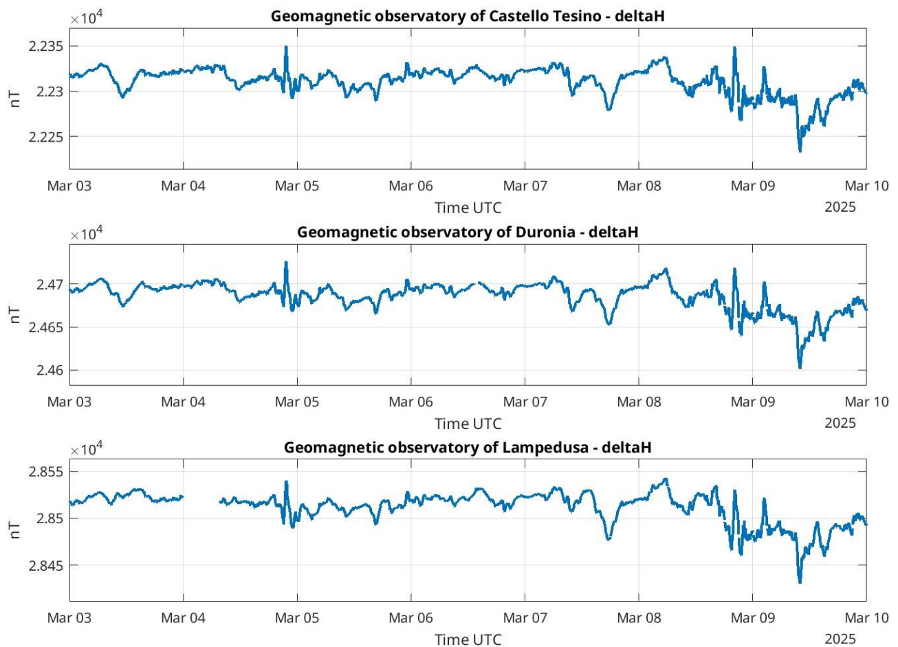
Figure 12: Magnetograms showing the variation of the horizontal component of the Earth's magnetic field at the Italian geomagnetic observatories (Castello Tesino, Duronio and Lampedusa from top to bottom).
