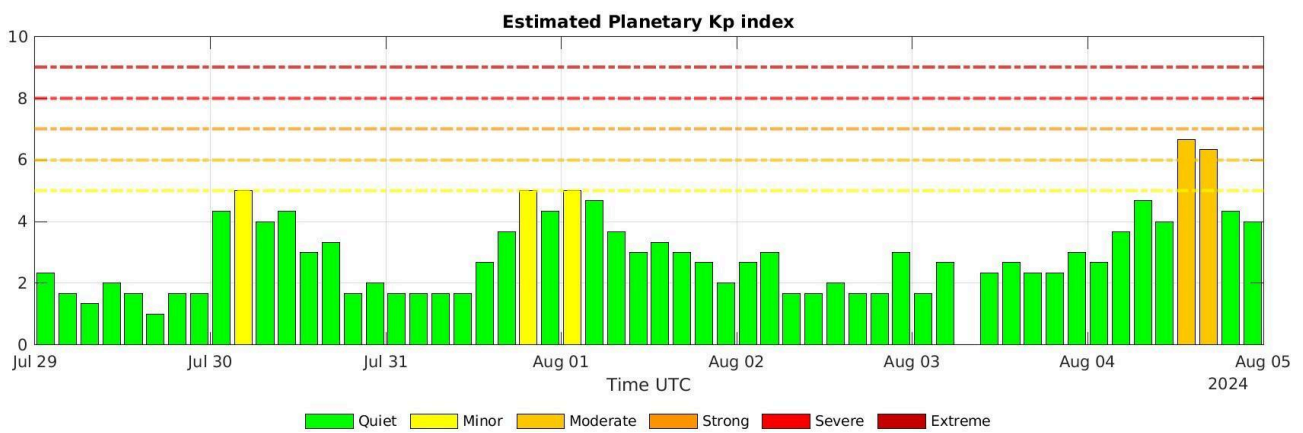
Figure 13: Histogram of Kp index released by NOAA. Coloured bars indicate the intensity of the global magnetic activity on Earth, according to the corresponding thresholds.
