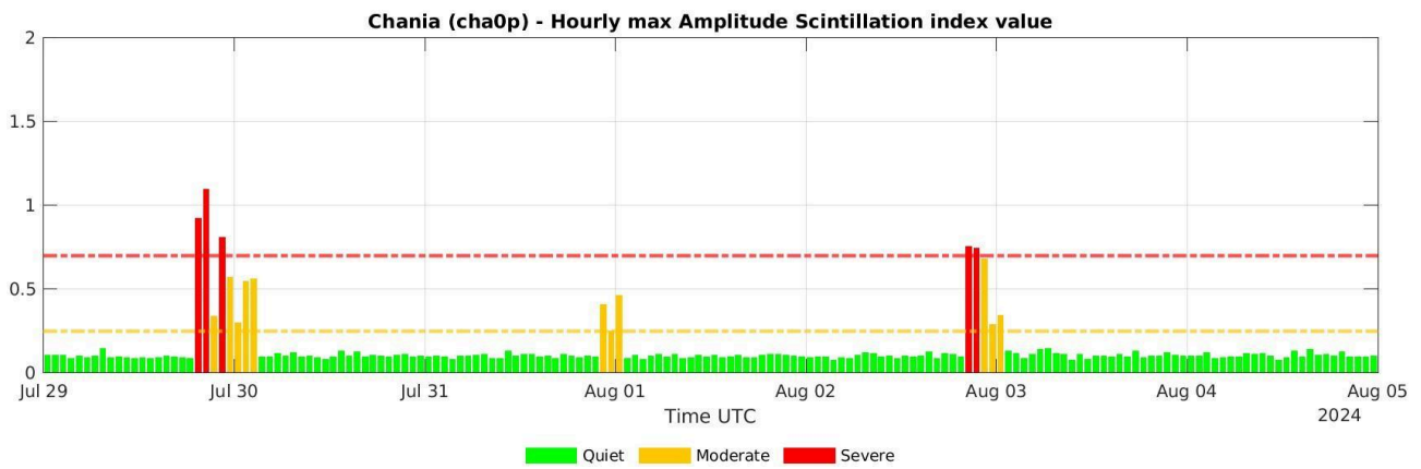
Figure 11: Same as Figure 9 for the data from the INGV receiver for GNSS scintillation located in Chania.
