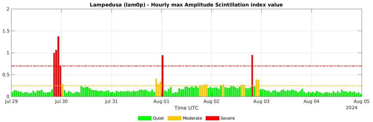
Figure 9: S4 hourly maximum values recorded by the INGV receiver for GNSS scintillation located in Lampedusa, with colors (green, yellow and red) associated to the severity of the scintillation, according to the 0.25 and 0.7 thresholds reported with horizontal yellow and red dashed lines, respectively.
