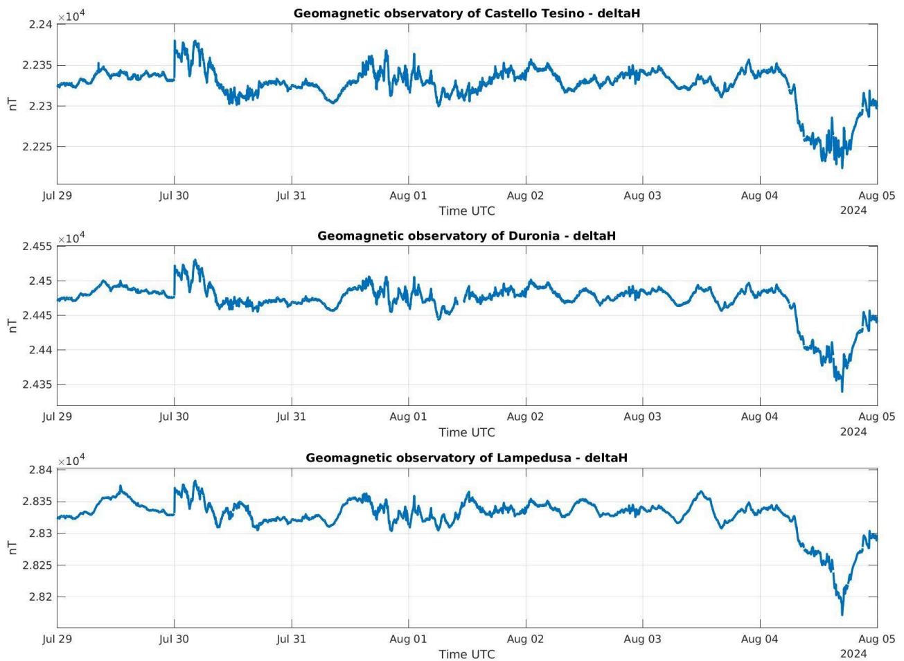
Figure 12: Magnetograms showing the variation of the horizontal component of the Earth's magnetic field at the Italian geomagnetic observatories (Castello Tesino, Duronia and Lampedusa from top to bottom).
