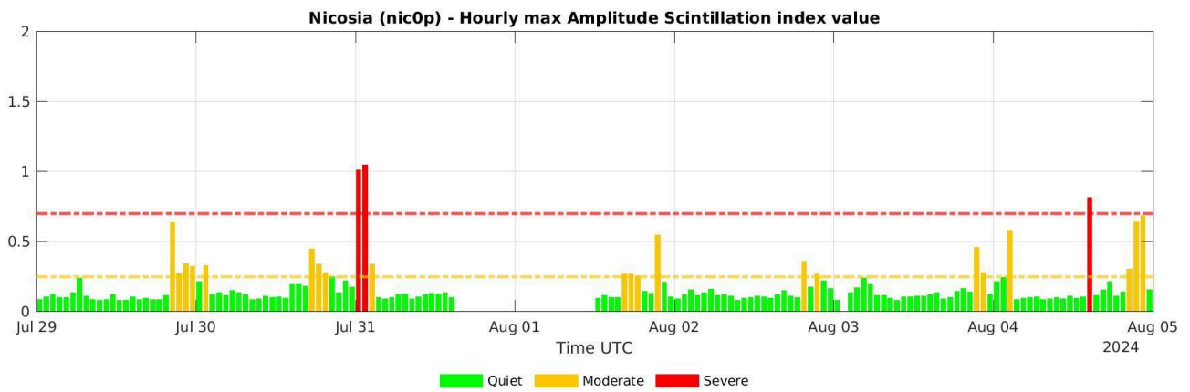
Figure 10: Same as Figure 9 for the data from the INGV receiver for GNSS scintillation located in Nicosia.
